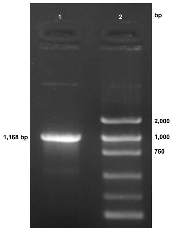
Figure 1 PCR amplification of HSV-TK gene from the pHSV-106 plasmid.
