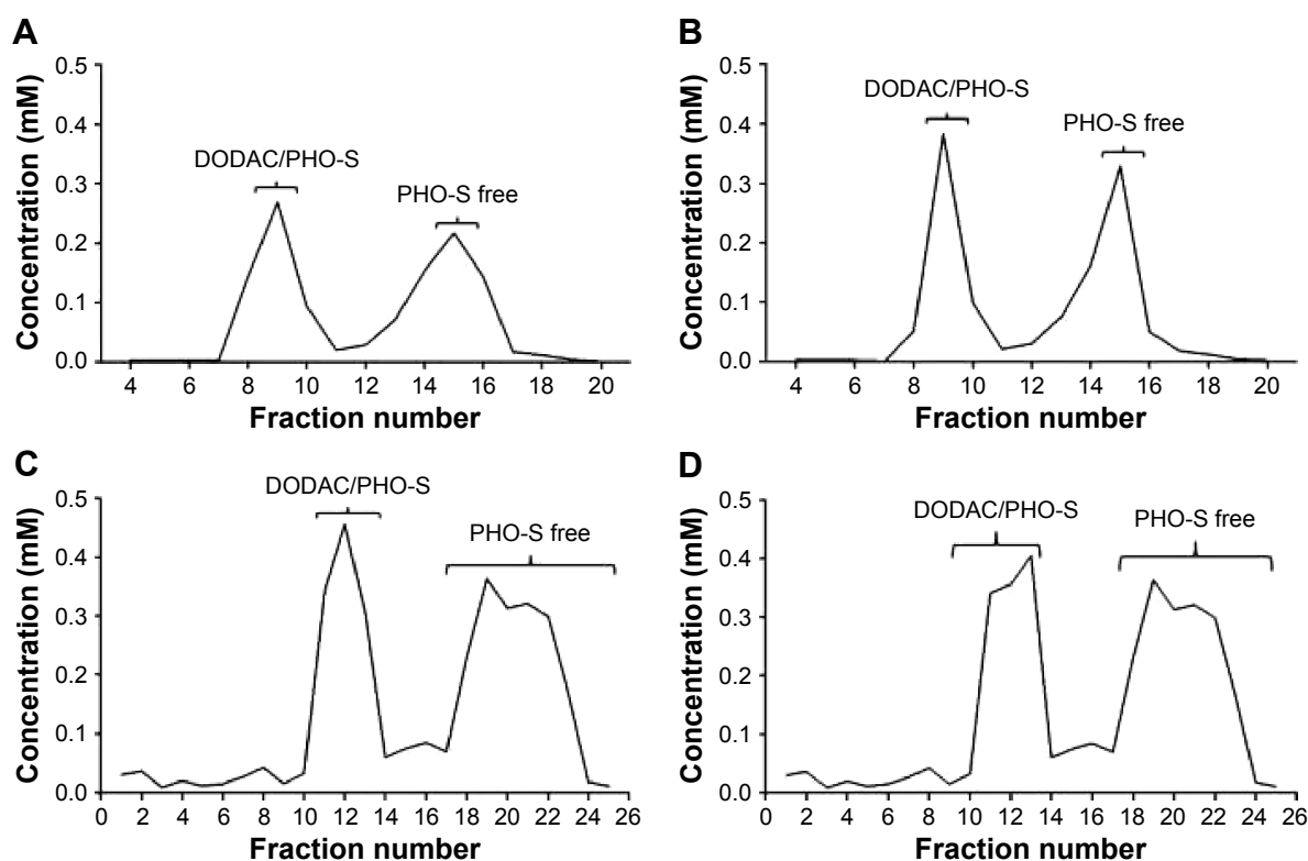
Figure 3 Chromatography of DODAC/PHO-S liposomal formulation.
