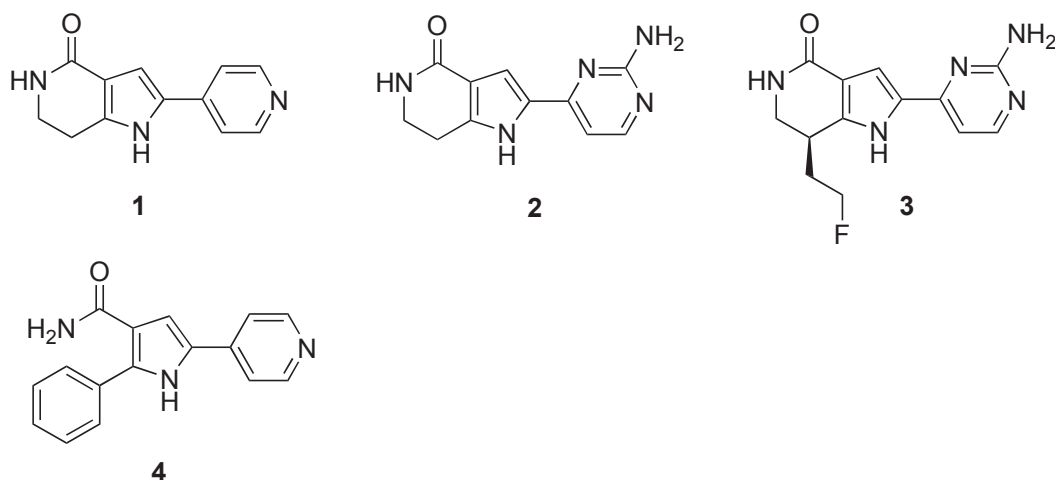
Figure 6 Cdc7 kinase inhibitors reported by Nerviano Medical Sciences. 1, PHA-767491 ( IC_{50} = 10 nM), 2, 3-aminopyrimidine analog ( IC_{50} = 7 nM), 3, (S)-2-(2-aminoimidin-4-yl)-7-(2-fluoroethyl)-1,5,6,7-tetrahydropyrrolo[3,2-c]pyridinone ( IC_{50} = 2 nM), and 4, the pyrrolopyridinone analog ( IC_{50} = 3 nM).
