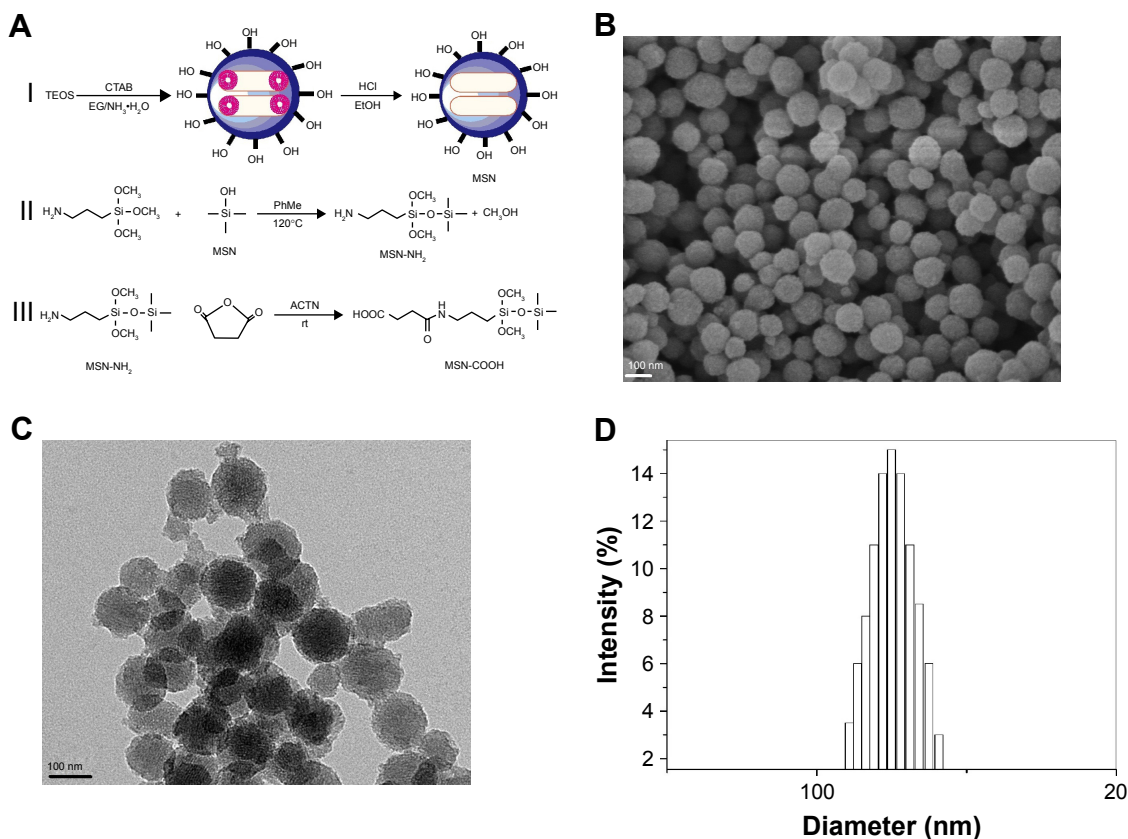
Figure 2 (A) Synthesis schemes of MSN (I), MSN-NH 2 (II), and MSN-COOH (III). (B) SEM images of MSN. (C) TEM images of MSN. (D) The size distribution of MSN determined by DLS (mean ± SD, n=5).
