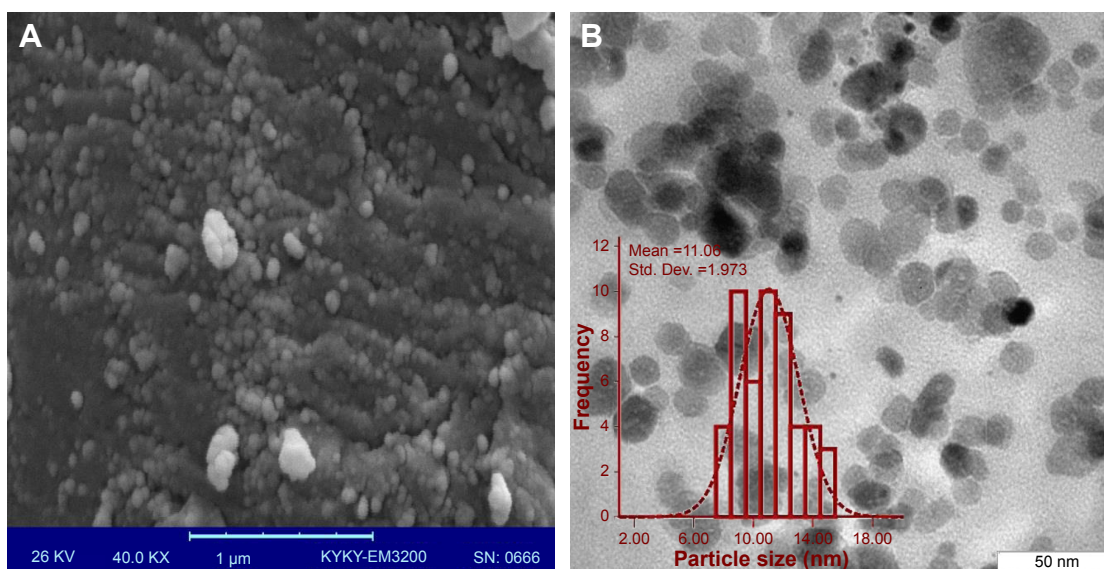
Figure 5 The (A) SEM and (B) TEM images, and particle size distribution (inset) of Pd@W.tea NPs. Abbreviations: Pd, palladium; SEM, scanning electron microscopy; Std. Dev., standard deviation; TEM, transmission electron microscopy; W.tea, white tea.
