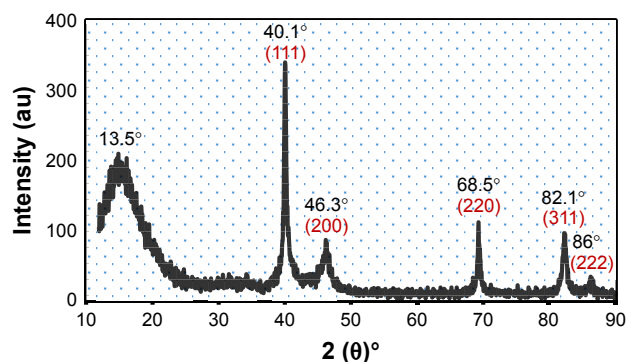
Figure 4 X-ray diffraction pattern of the Pd@W.tea NPs. Abbreviations: NPs, nanoparticles; Pd, palladium; W.tea, white tea.
