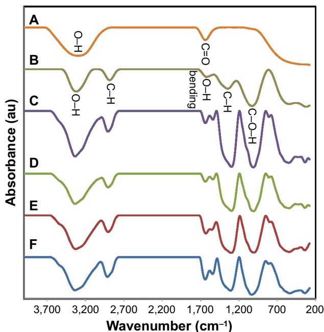
Figure 2 Fourier transform infrared spectra of (A) fruit extract, (B) pure BNC, and (C–F) BNC/Ag nanocomposites (16.0–1.0 wt%), respectively. Abbreviation: BNC, bacterial nanocellulose.
