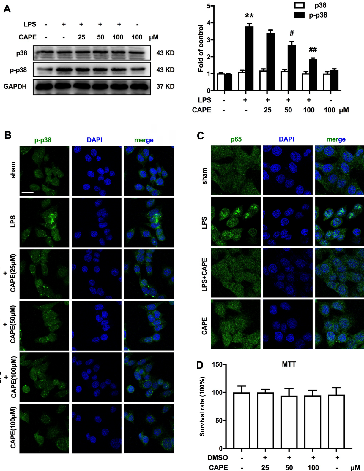
Figure 6 CAPE suppressed LPS-induced microglia activation by inhibiting p38 MAPK/NF-κB.
