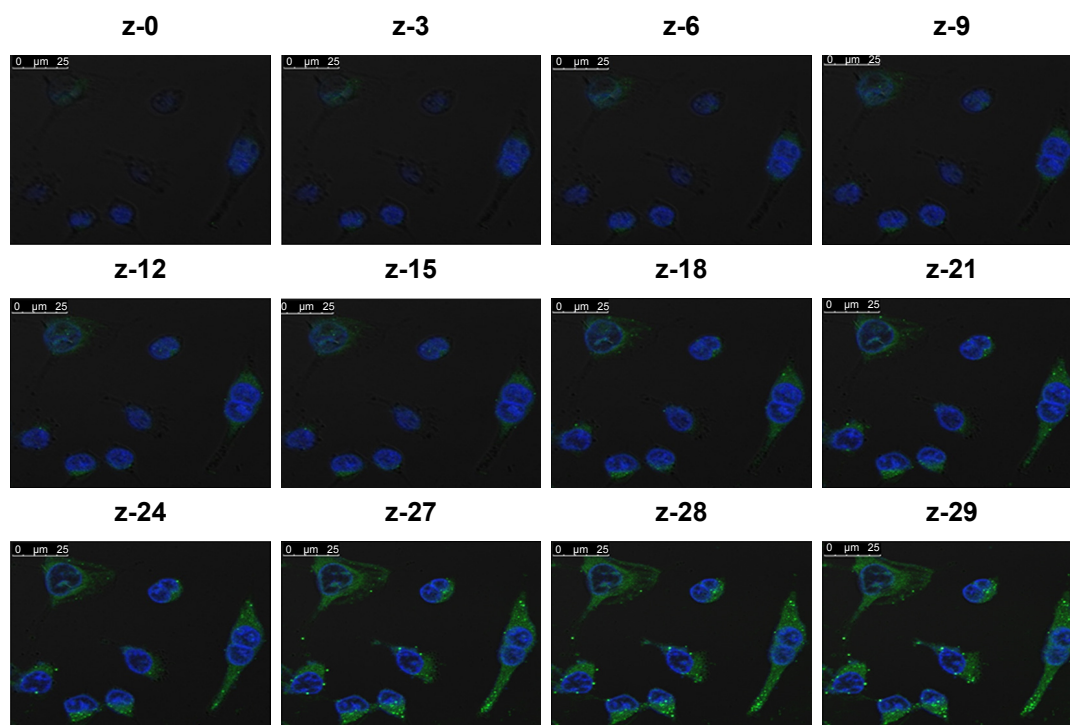
Figure S3 Live uptake of ion-paired LCNPs in A549 cells in which three-dimensional time laps images distinguishing between cytosolic and perinuclear accumulation of 178 nm LCNPs of 30 z-stacks inside the cells in the z-direction along the total depth measured (z-stack = 30 slices at 25 \mu\text{m} per slices).
