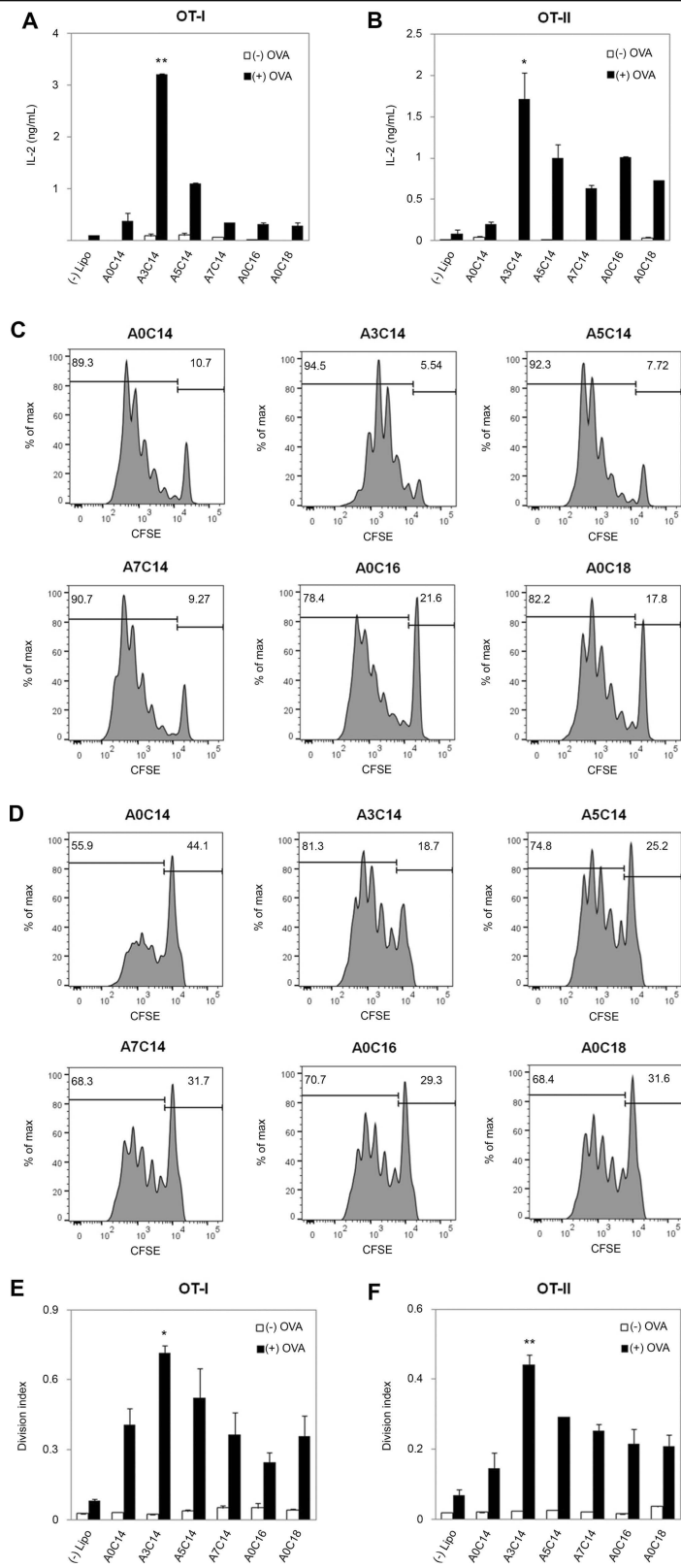
Figure 5 Activation of OT-I and OT-II cells through MHC-I and MHC-II mediated antigen presentation pathways, respectively. BMDCs were incubated with OVA (fc: 25 μg/mL)-loaded cationic liposomes (fc: 25 μM) or the same concentration of soluble OVA, or the same concentration of liposomes for 2 hrs, and then extracellular OVA or liposomes were washed off with DPBS. CFSE was used to label splenocytes from OT-I mice ( A, C, E ) or OT-II mice ( B, D, F ) and then labeled cells were added into the BMDC culture plate. The supernatant was partially collected after overnight incubation to detect the secretion of IL-2 using an ELISA kit ( A, B ); and the cells were collected after 48 hrs incubation to analyze the OT-I cell and OT-II cell division using flow cytometry ( C, D, E, F , see gating strategies of OT-I and OT-II cells in Figure S5). (-) Lipo indicates the BMDCs without treatment [(-) OVA] or treated with soluble OVA [(+) OVA]; other experimental groups were treated with naked liposomes [(-) OVA], or OVA-loaded liposomes [(+) OVA]. Data show the mean±SD of two independent experiments with two replicates, respectively; *P<0.05, **P<0.01.
