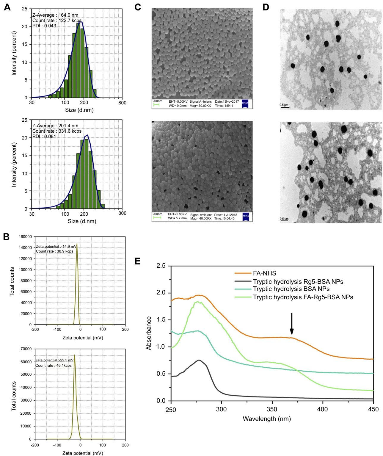
Figure 2 (A) Hydrodynamic size distributions, (B) Zeta potentials, (C) SEM and (D) TEM images of Rg5-BSA NPs (top) and FA-Rg5-BSA NPs (bottom), and (E) UV-vis absorption spectra determining the amount of FA in Rg5-BSA NPs.
