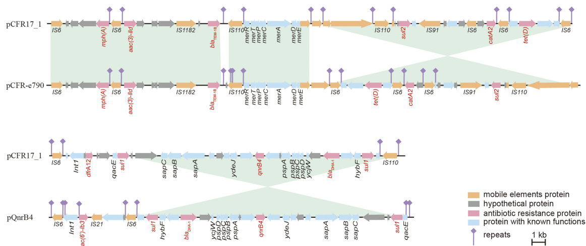
Figure 2 Lineal comparison of multidrug-resistant regions of pCFR17_1, pCFR-e790 and pQnrB4. Genes were portrayed by arrows and colored according to their functions.
