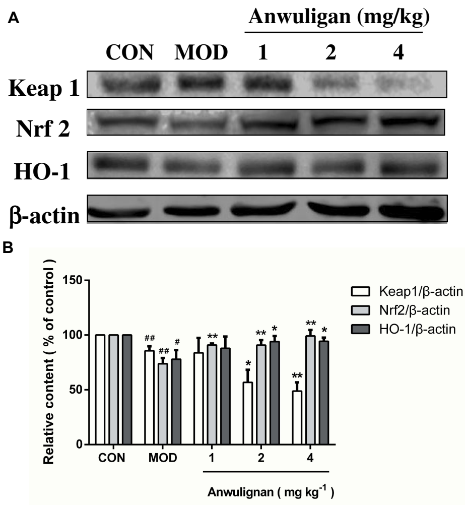
Figure 7 Effects of Anwuligan on the expressions of Keap1, Nrf2, and HO-1 proteins in the spleen cells of mice (mean±SD, n=3).
