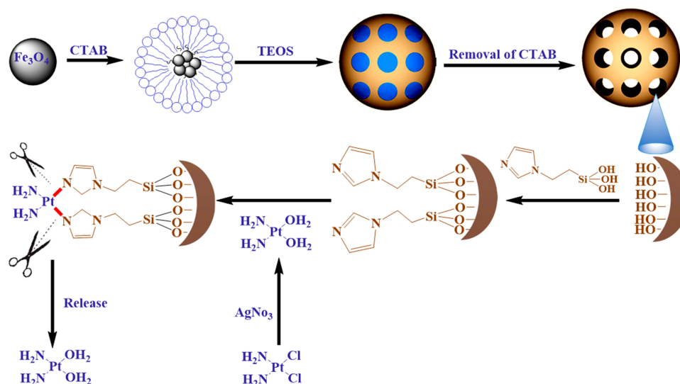
Figure 1 Schematic representation of the preparation of magnetic mesoporous silica nanoparticles functionalized with TIP (MMSN-Imi) for subsequent loading and release of aquated cisplatin.
