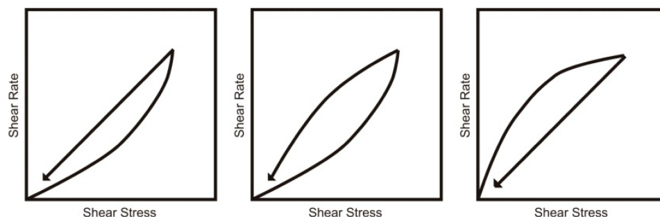
Figure 3 Thixotropic in pseudoplastic, plastic, and dilatan systems.
