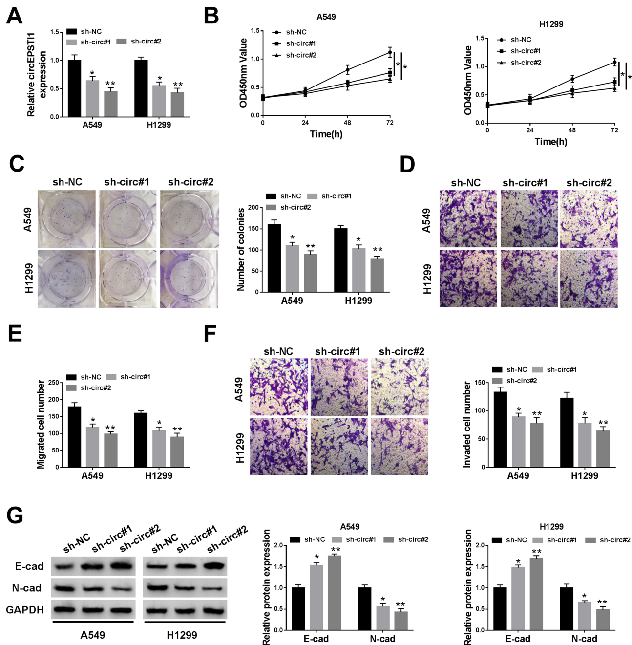
Figure 2 CircEPSTII accelerates the proliferation, colony formation and metastasis of NSCLC cells in vitro. A549 and H1299 cells were transfected with sh-circ#1 or sh-circ#2 to establish NSCLC cell lines stably knockdown circEPSTII, and sh-NC group was the control group. (A) The knockdown efficiency of circEPSTII was evaluated in the above A549 and H1299 cells by qRT-PCR. (B) CCK8 assay was applied to detect the proliferation of NSCLC cells transfected with sh-NC, sh-circ#1 or sh-circ#2. (C) The capacity of colony formation in NSCLC cells transfected with sh-NC, sh-circ#1 or sh-circ#2 was evaluated by colony formation assay. (D-F) The abilities of migration and invasion in A549 and H1299 cells were assessed by transwell assays. (G) The expression of E-cad and N-cad was measured in A549 and H1299 cells by Western blot assay. *p<0.05, **p<0.01.
