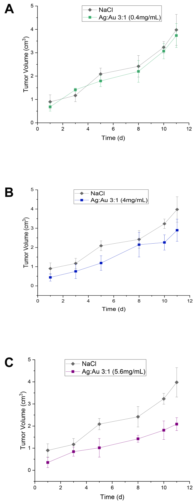
Figure 3 Effect of intratumoral injection of \text{Ag}_3\text{Au}_1\text{Trp}_{1,2} NPs (three different concentrations) or normal saline on the Tumor Volume of 4T1 tumor-bearing SCID mice. Values represent the mean \pm SD ( n = 3 mice per group). (A–C) show the difference in tumor volume of each concentration of \text{Ag}_3\text{Au}_1\text{Trp}_{1,2} NPs in direct comparison to the Control Group (untreated).
