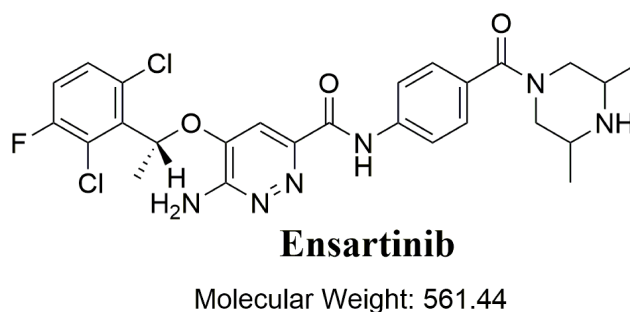
Figure 1 Chemical structure of ensartinib.
