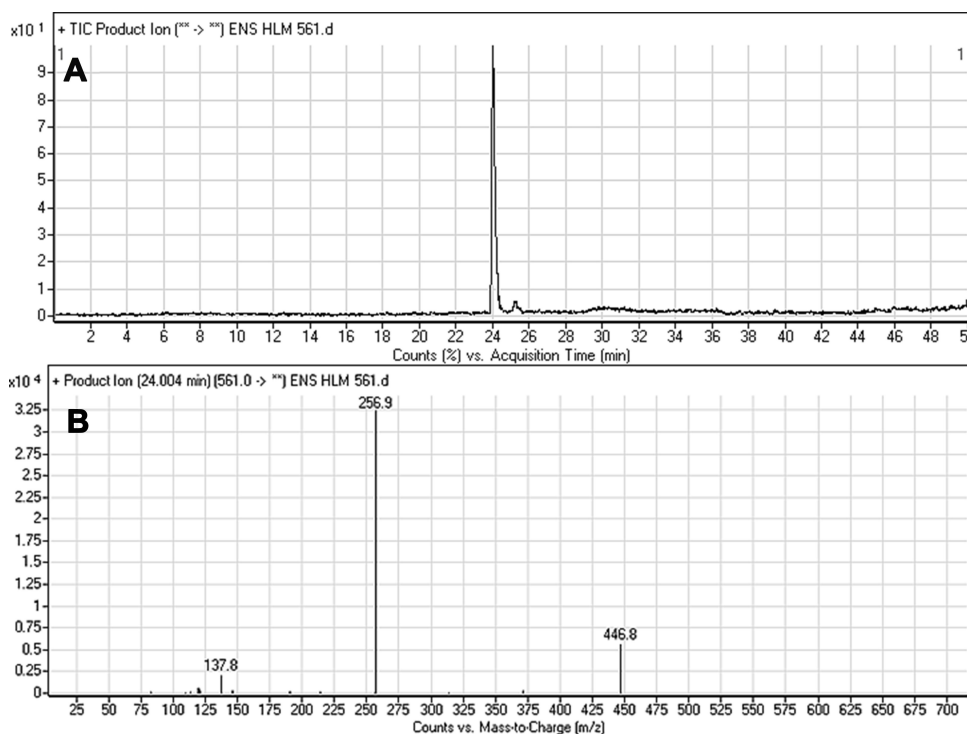
Figure 4 Fragment ion (m/z 561) chromatogram displaying the ESB peak at 24.0 min (A). Fragment ions of ESB (B).
