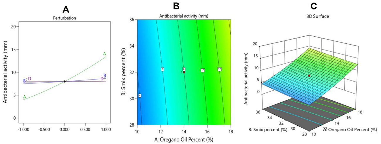
Figure 4 Main effect (A), contour (B), and 3D surface (C) outlines illustrating the effects of different factors on response Y_3 (antibacterial activity) of various OEO-SNEDDSs.
