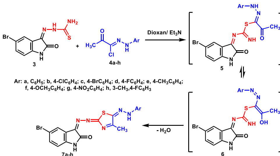
Scheme 2 Synthesis of isatin-decorated thiazole derivatives 7a-h.
