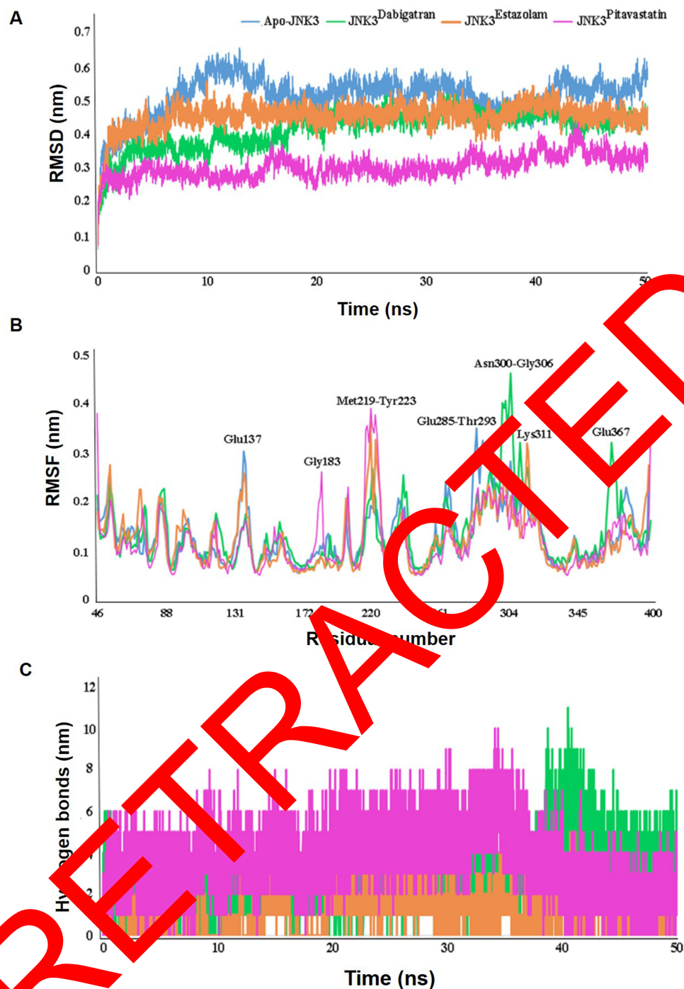
Figure 4 Time-dependent analysis of MD trajectories of apo and inhibitor bound states of JNK3. (A) RMSD plots were made via the least square fitting method using the backbone of the \alpha -carbons. (B) Relative RMSF plot of apo-JNK3 (blue), JNK3 Dabigatran (green), JNK3 Estazolam (orange), and JNK3 Pitavastatin (pink). (C) Time versus intermolecular hydrogen bonding pattern for the 50 ns MD simulation.
