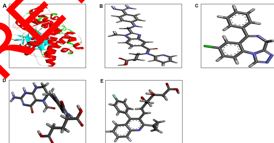
Figure 1 The 3D structure of protein and ligand molecules (A) JNK3 (PDB ID: 3TTI). Structures of the selected FDA approved drugs (B) dabigatran, (C) estazolam, (D) leucovorin, and (E) pitavastatin.
