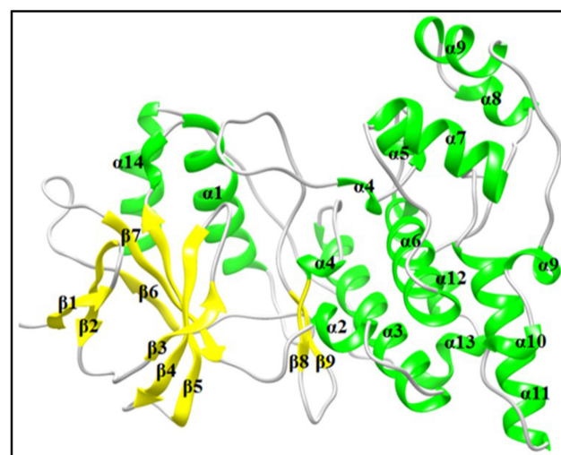
Figure 3 The refined 3D structure of JNK3. The 3D structural architecture of JNK3 is shown. \alpha -helices and \beta -sheets are colored in green and yellow, and the linker region is colored in gray.
