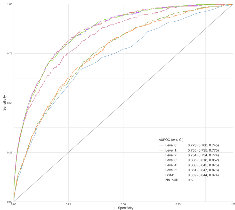
Figure 2 Receiver-operating characteristic curves and appertaining area under curve for the seven models when evaluated on the test set. Abbreviations: AUROC, area under receiver-operating characteristic curve; BSM, backward-selection model.
