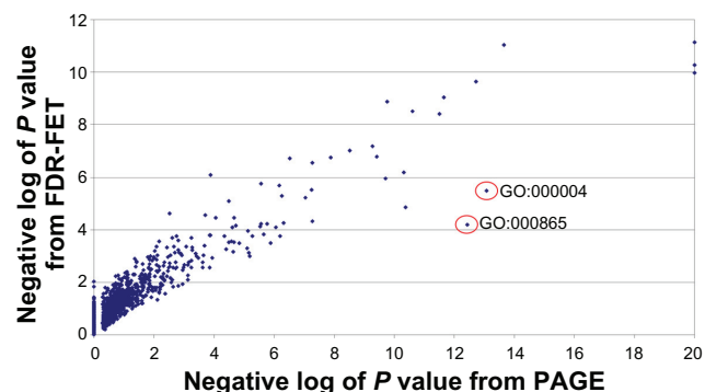
Figure 3. Comparison of the analysis result of FDR-FET with that of PAGE. P values are calculated for gene sets from the Gene Ontology and KEGG for the human immunodeficiency virus protease inhibitor experiment using FDR-FET (with the option “genes” and maximal FDR 35%) and PAGE (using the whole vector of gene P values as input). Gene sets of size \geq 10 are included in the plot.
